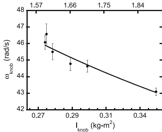
Fig. 7 Plot of the angular velocity \omega_{\text{knob}} of the bat about the knob just prior to impact versus the I_{\text{knob}} , the MOI of the bat about the knob. Each point represents the angular velocity of a given bat, averaged over all impacts, as determined from Gaussian fits, with values given in Table 2. The curve is a power-law fit of the form \omega_{\text{knob}} \sim 1/I_{\text{knob}}^n , with n = 0.29 \pm 0.04 . The upper horizontal scale is I_{\text{knob}} in units of 10^4 oz in. 2
