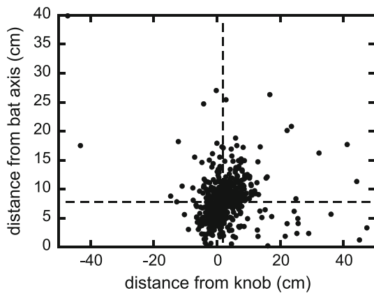
Fig. 5 Composite scatter plots for all bats and all impacts showing the instantaneous rotation axis of the bat just prior to the collision, plotted as the off-axis ( x ) versus the on-axis distance ( z ). The latter is measured from the knob of the bat and the former is positive when pointed towards the catcher. The dashed lines show the mean distances, with an intersection at z = 1.65 cm (0.65 in.) and x = 7.5 cm (3.0 in.), corresponding approximately to the location of the wrist of the bottom ( left ) hand of the right-handed batters
