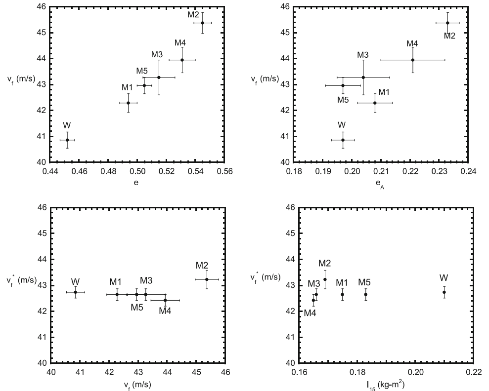
Fig. 3 Correlations between v_f and e ( upper left ), v_f and e_A ( upper right ), v_f^* and v_f ( bottom left ), and v_f^* and the swing weight I_{15} ( bottom right )
