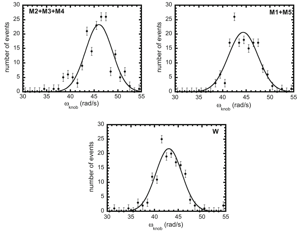
Fig. 6 Histograms of the angular velocity of the bat about the knob just prior to impact, where bats with similar values of MOI have been grouped together. A Gaussian fit to each histogram, shown as the curve, results in the values of \omega_{\text{knob}} presented in Table 2 and plotted against I_{\text{knob}} in Fig. 7
