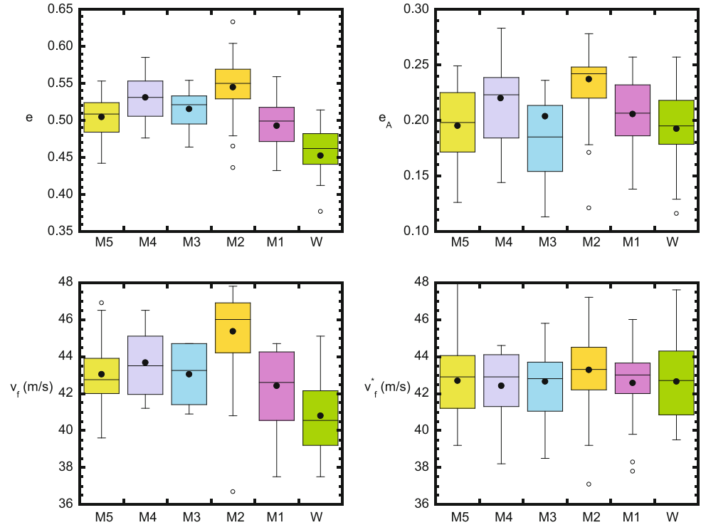
Fig. 2 Box plot of the BBCOR ( upper left ), collision efficiency ( upper right ), and ball exit velocities v_f ( lower left ) for hits in the impact range 8.9–19.1 cm (3.5–7.5 in.) from the barrel end of the bat. For each bat, the closed point represents the mean value, the horizontal line is the median value, and the shaded region is bounded by the upper quartile ( U ) and lower quartile ( L ), with the interquartile distance D equal to U - L . The flags are the bounds of points within the range (L - 1.5D) – (U + 1.5D) , while the open points are events lying outside those bounds. The lower right panel is a box plot of the adjusted ball exit velocity v_f^* , which is calculated from Eq. 5. Differences in v_f^* among the bats are due entirely to differences in inertial factors rather than to differences in e
